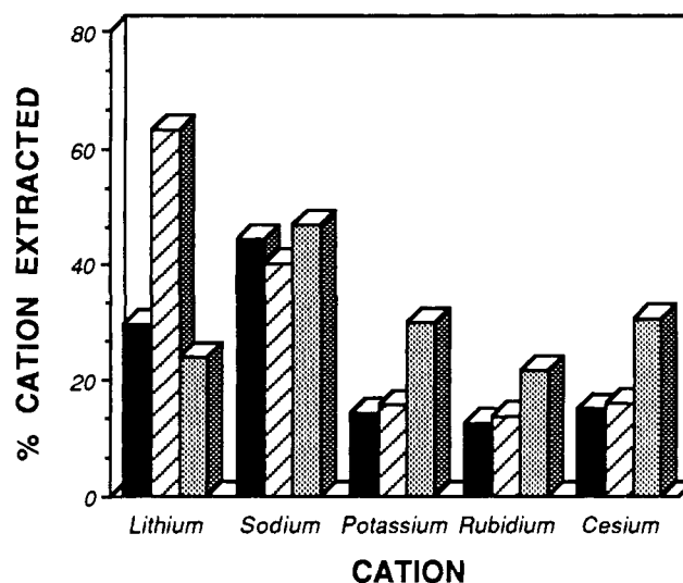
Figure 2. Extent of alkali metal ion extraction by complexes 4 , 5 , 6 , and 6 , at 25 ± 5 °C. Aqueous phase: [M + Picrate - ] = 7.5 mM. Chloroform phase: [host] = 2 mM. Values are averages of at least two independent determinations. All values are reproducible to within 5%.
